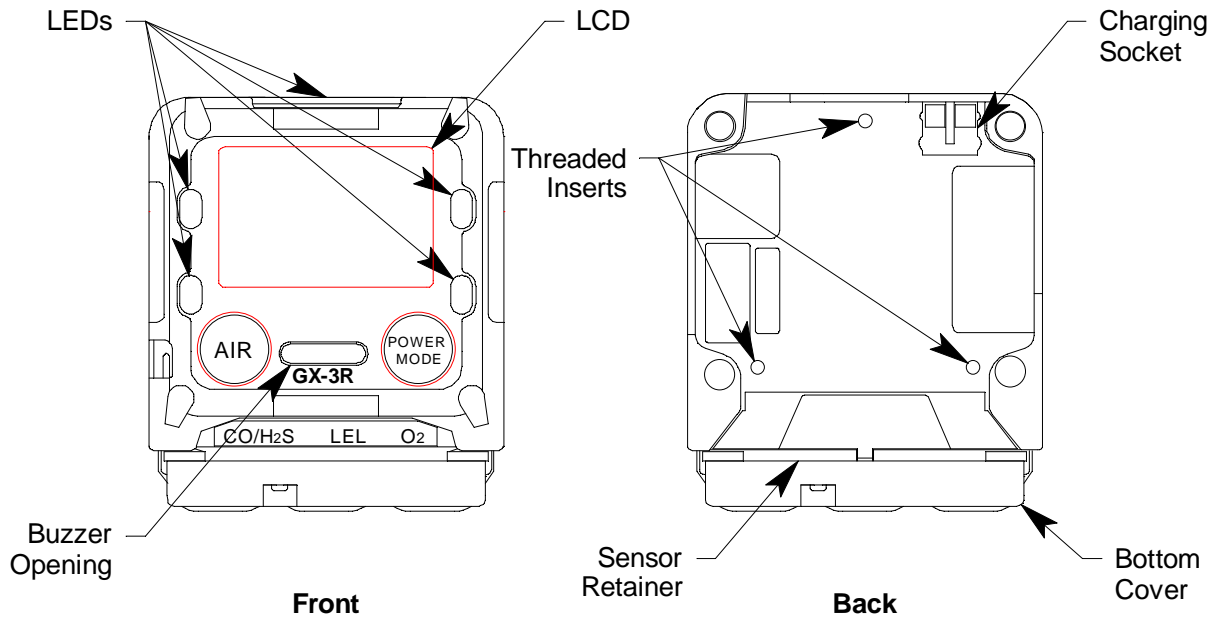
Figure 1: Component Location
