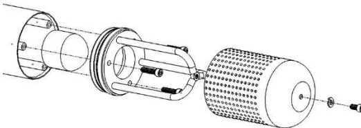
Figure 7-3: 4" Screened Intake
