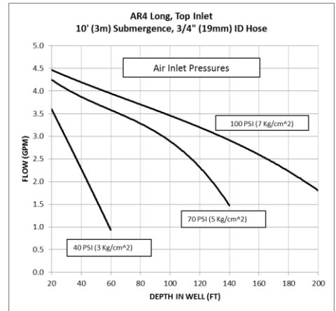
Figure 4-8: AR4 Long Bottom/Top Inlet 10' (3 m) Submergence, 3/4" (19 mm) ID Hose in GPM
