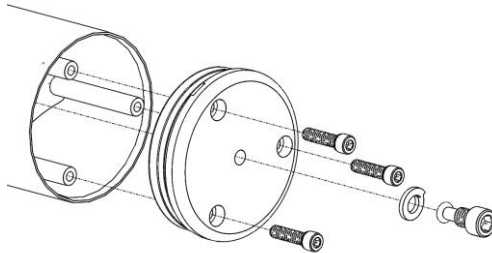
Figure 7-1: Blank Bottom Cap
