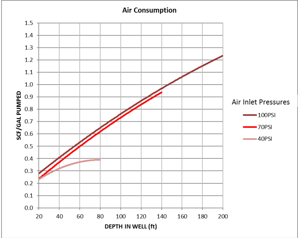
Figure 2-4: Air Consumption
